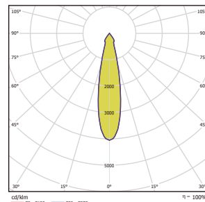
CURVA POLAR SPOT
