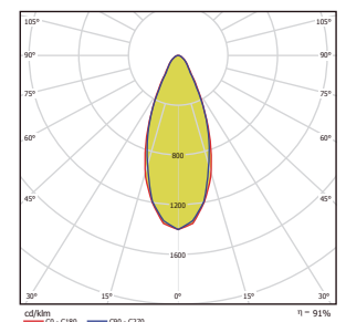
CURVA POLAR FLOOD
