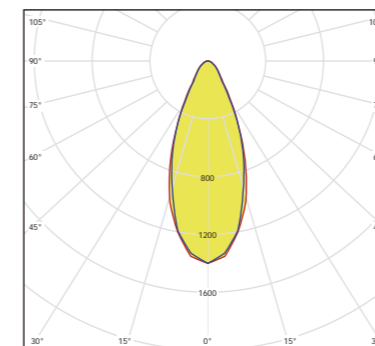
CURVA POLAR FLOOD
