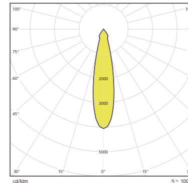
CURVA POLAR SPOT
